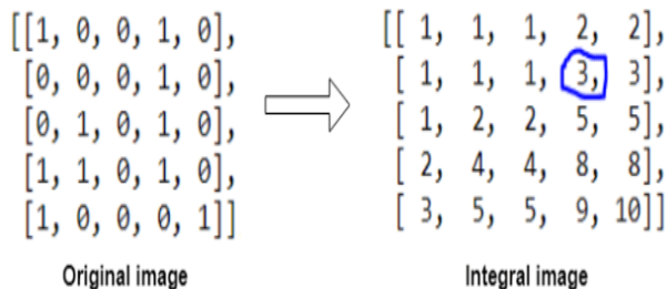
Fig 3: Integral Image
