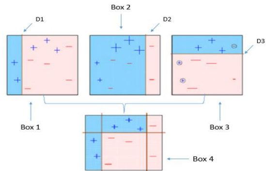
Fig 4: AdaBoost Classifiers
