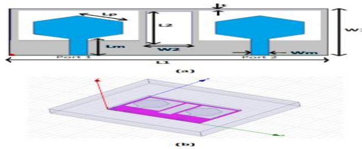
Fig.1. Proposed 2×2 MIMO Antenna (a) UPPER SURFACE showing patch with the ground structure, (b) HFSS mode
