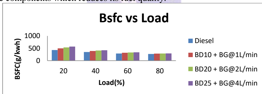
Fig.7 Variation of brake specific fuel consumption with respect to engine load
