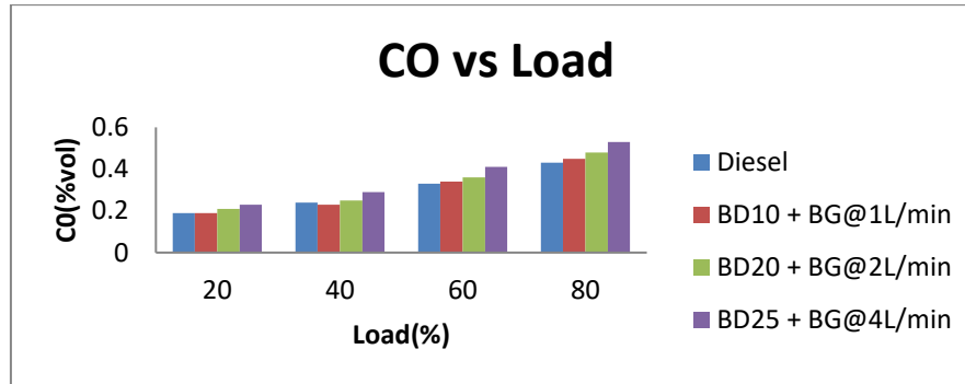
Figure 8 Variation of CO emissions with respect to load
