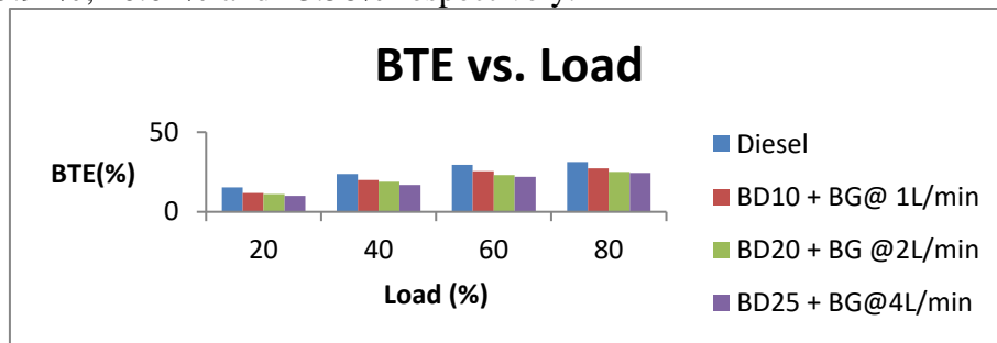
Fig. 6 Variation of brake thermal efficiency versus engine load.
