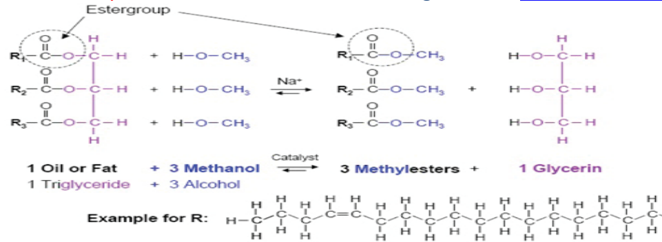
Fig 4 Transesterification of oil and fat
