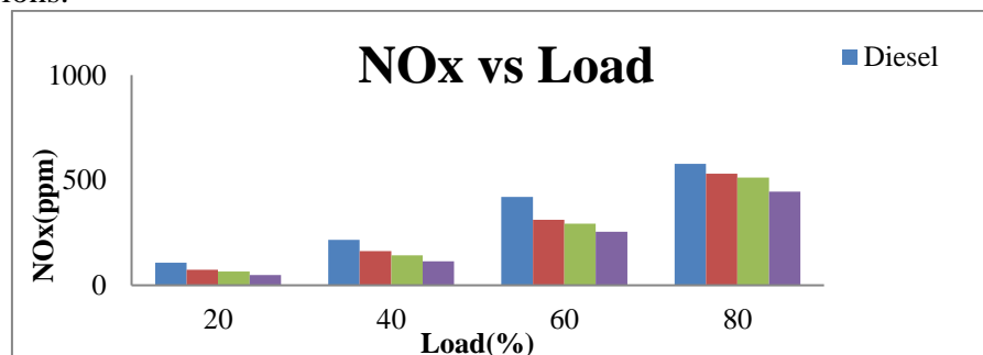
Fig.18 Variation of NOx emissions with respect to load
