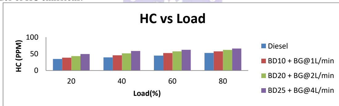
Figure 9 Variation of HC emissions with respect to load
