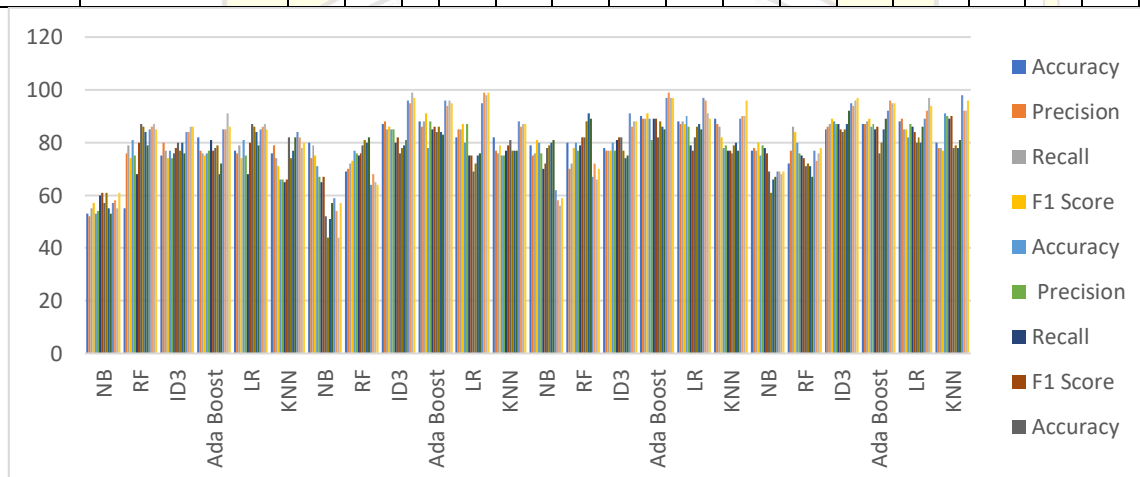
Figure 3: Measuring Performance of Various Attacks in KDD CUP 99 Dataset
