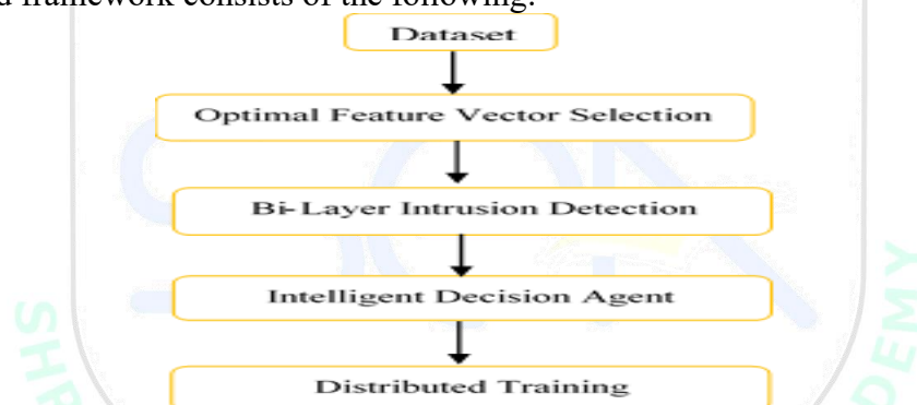
Figure 1: Proposed Framework
