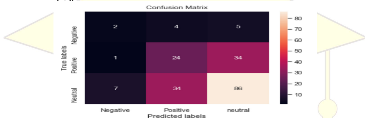
Figure 4: Confusion matrix
