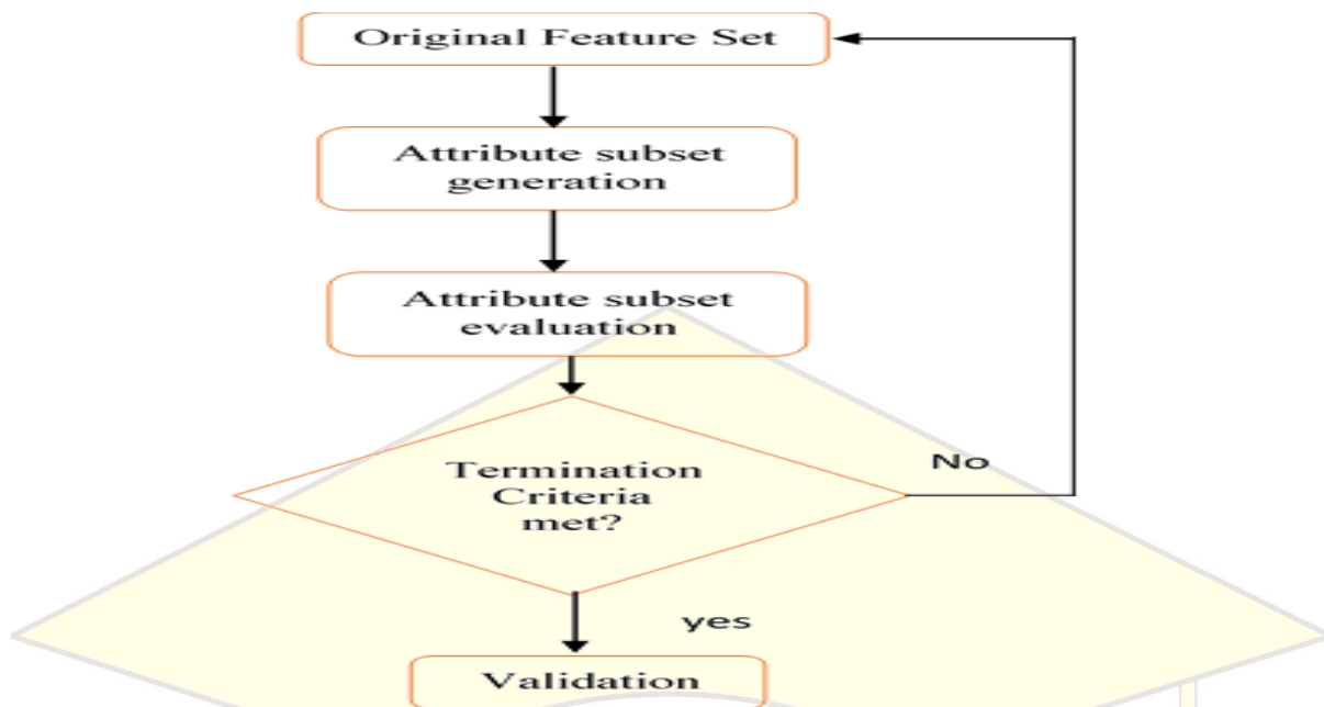
Figure 2: Steps in Feature Selection
